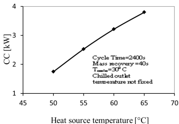
Figure 2. The effect of heat source temperature on CC
