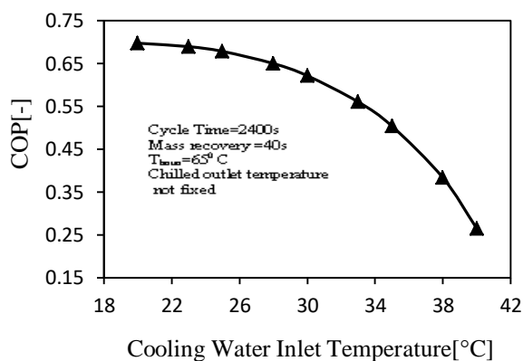
Figure 5. The effect of cooling water inlet temperature on COP
