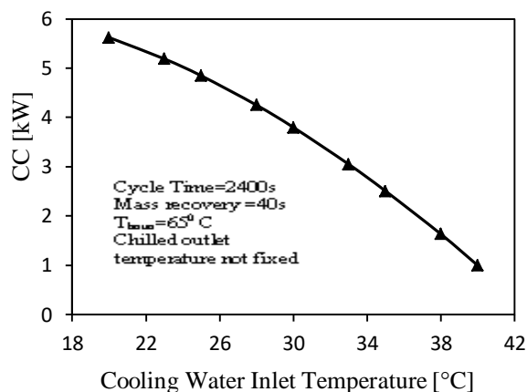
Figure 4. The effect of cooling water inlet temperature on CC
