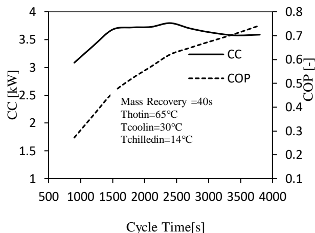
Figure 6. Cycle time effect on CC and COP
